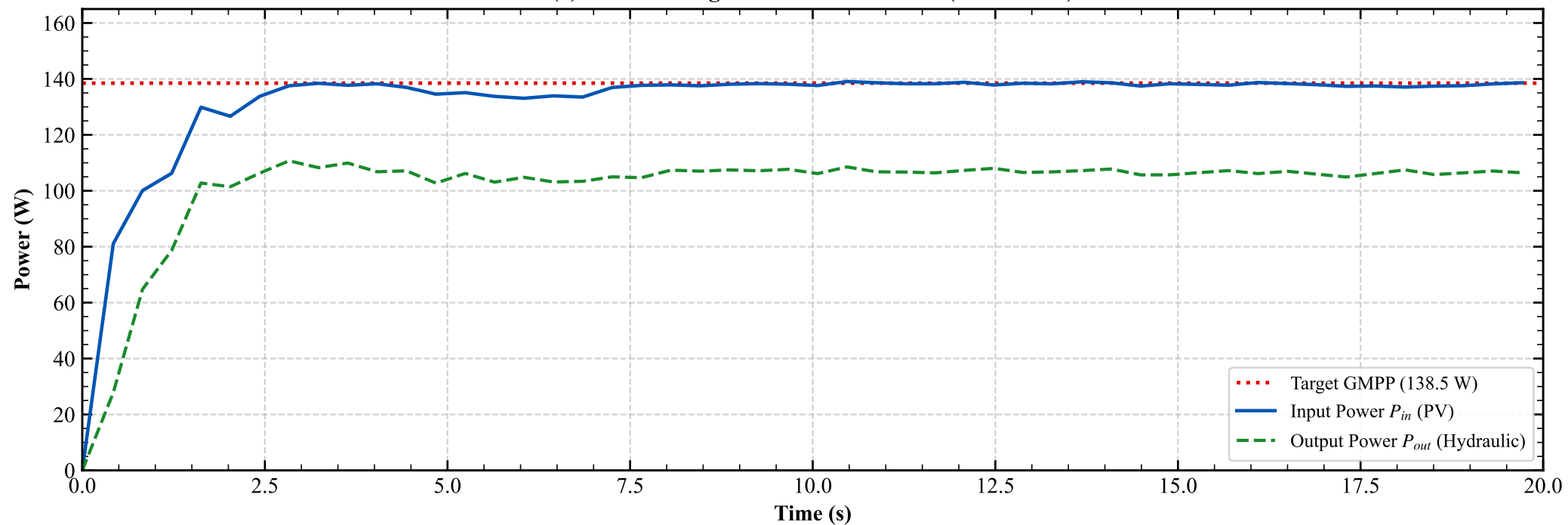
(b) Shading Condition — Level 2 (660 W/m 2 )
